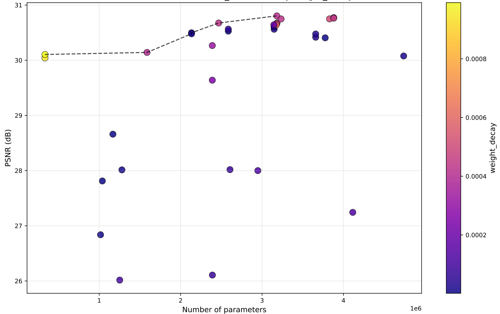
PSNR vs #Params — DHTCUN_baseline — by weight_decay
